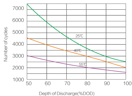
Cycle life versus DOD and temperture at 0.2C
