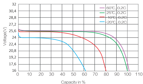
Dis charge curves under differents temperatures
