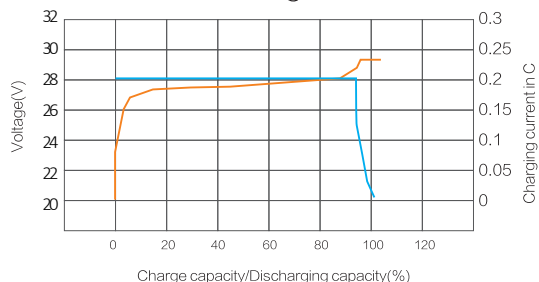
0.2C CC-CV charge characteristic
