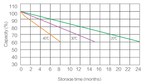
Self-discharge characteristic
