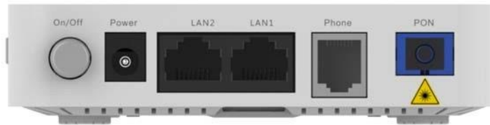
Figure 2-15 Rear Panel of the AN5506-02-B
