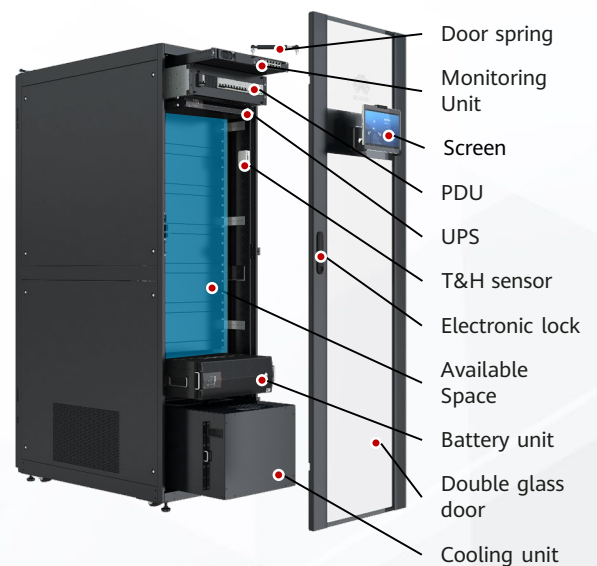
FusionModule500 Architecture
